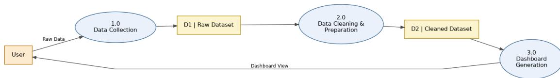
Figure 6.5 – DFD Level 1
